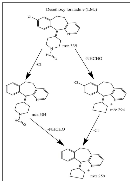
Fig 13: Mass fragmentation pattern of Loratadine metabolite, LM2
