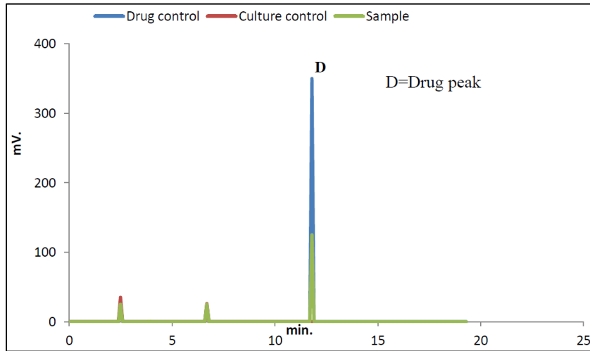
Fig 5: HPLC chromatogram of Loratadine from culture extracts of Cunninghamella blackesleena
