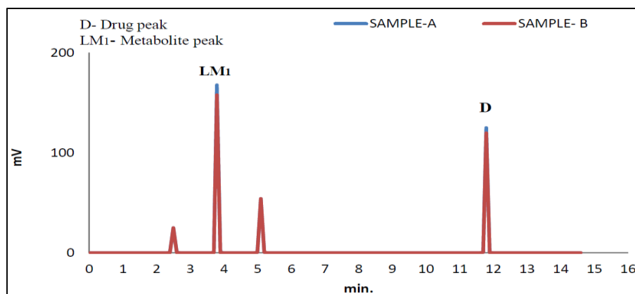
Fig 20: HPLC chromatogram of Loratadine in the presence of Carbamazepine from culture extracts of Cunninghamella elegans (CYP3A4 induction study)
