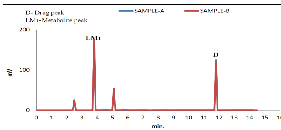
Fig 21: HPLC chromatogram of Loratadine in the presence of Fluoxetine from culture extracts of Cunninghamella elegans (CYP 3A4 inhibition study)
