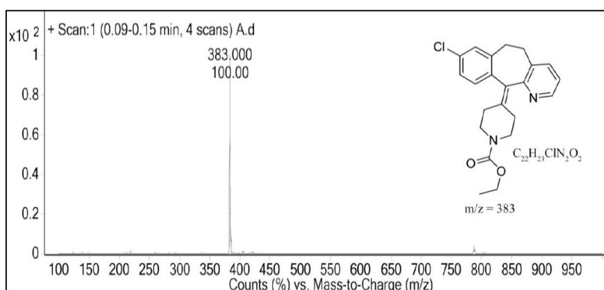
Fig 9: Mass spectrum of Loratadine
