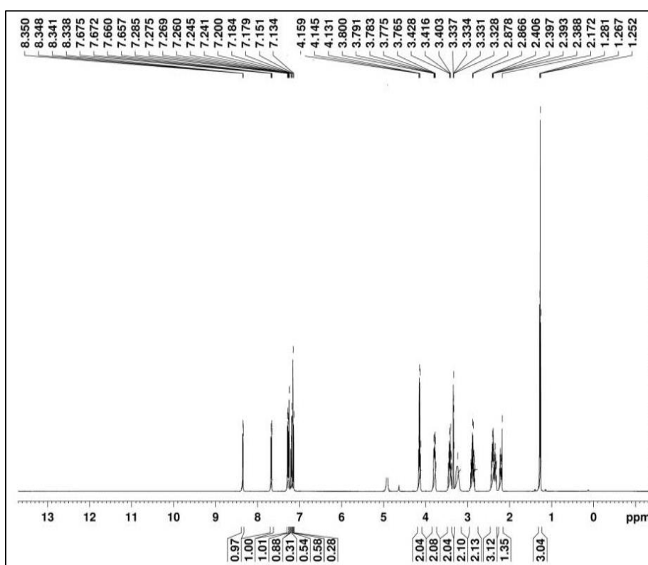
Fig 16: 1 H NMR spectrum of Loratadine
