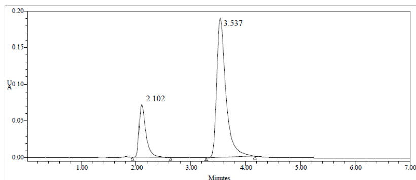
Fig 3: Optimized Chromatographic Condition
