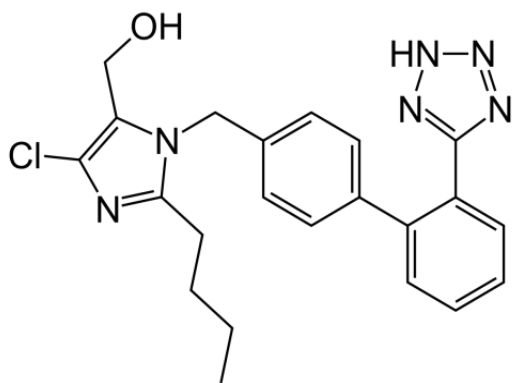
Fig 1: Chemical Structure of Losartan
