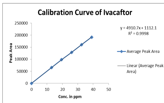
Fig 6: Calibration Curve of Ivacaftor
