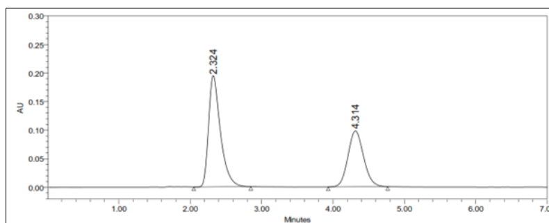
Fig 4: Chromatogram of Optimized Method
