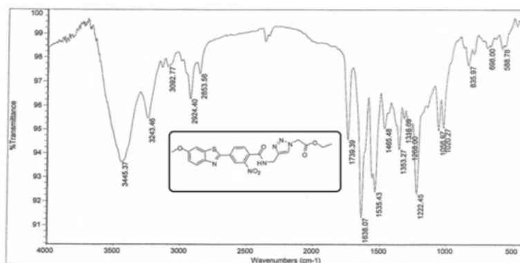
IR spectrum of compound 10b
