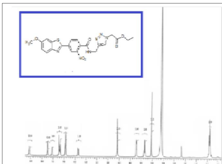
1 H NMR spectrum of compound 10b
