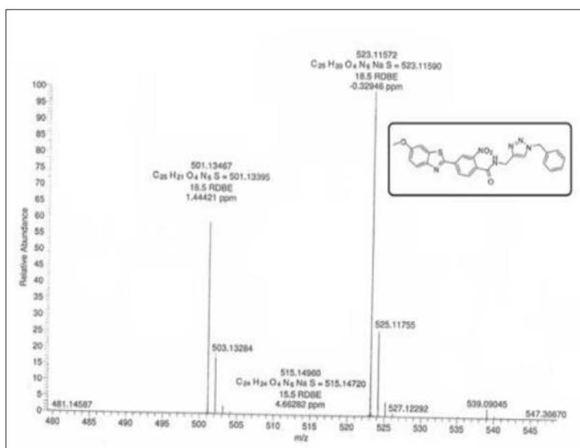
ESI-MS spectrum of Compound 10a
