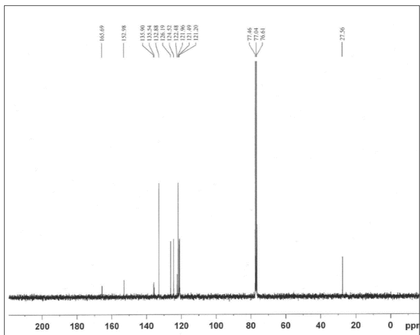
13 CNMR spectrum of compound 13
