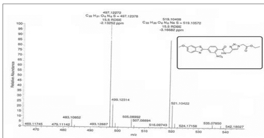
ESI-MS spectrum of compound 10b
