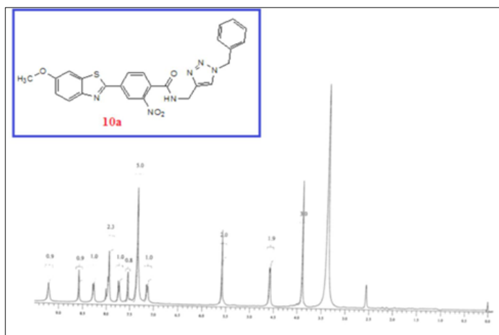
Compound 10a: 1 H NMR
