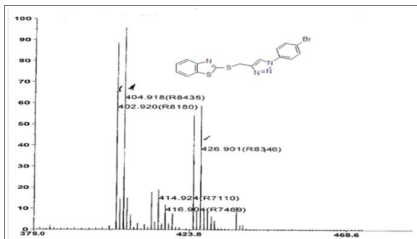
Mass spectrum of compound 13
