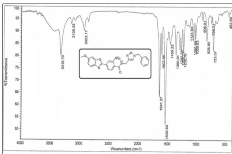
IR Spectrum of Compound 10a
