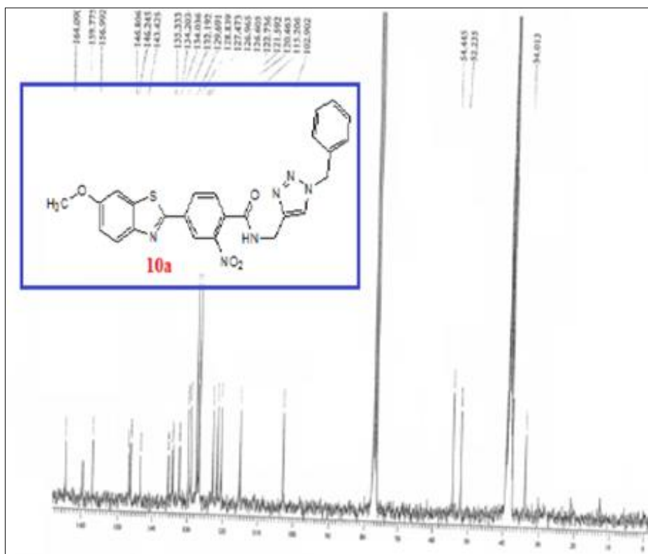
13C NMR Spectrum of Compound 10a
