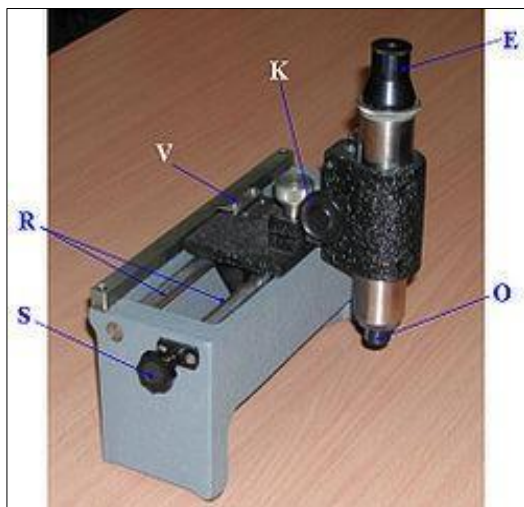
Fig 5: Travelling Microscope
