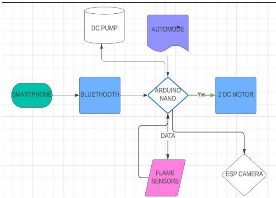
Fig 1: Block diagram of Fire Fighting Robot
