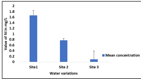
Fig 1: Fluctuations of Iron in waters samples
