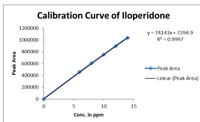
Fig 3: Calibration Curve of Iloperidone
