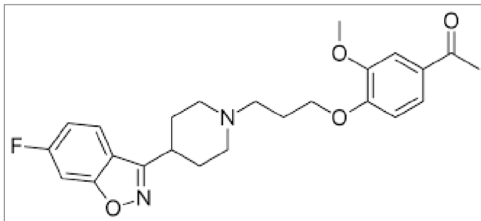
Fig 1: Chemical Structure of Iloperidone
