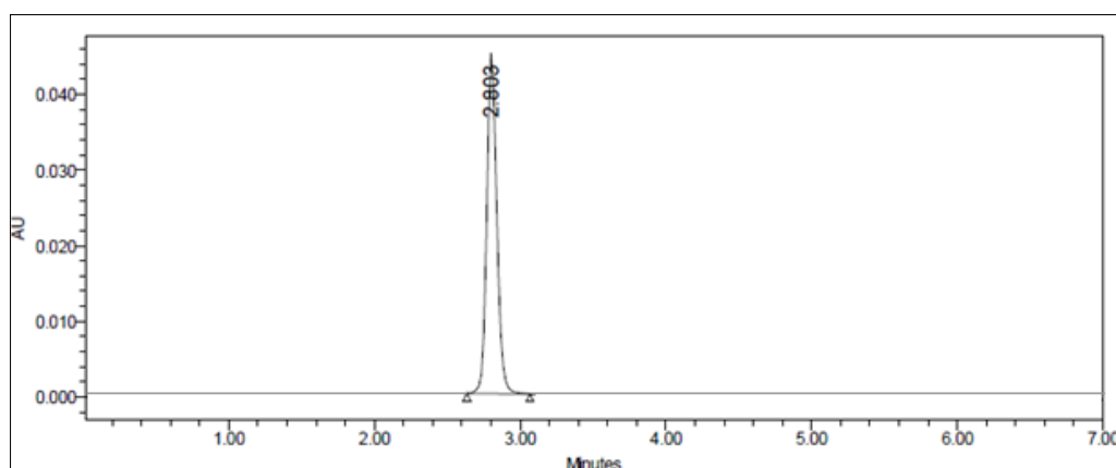
Fig 2: Optimized Chromatogram for Iloperidone
