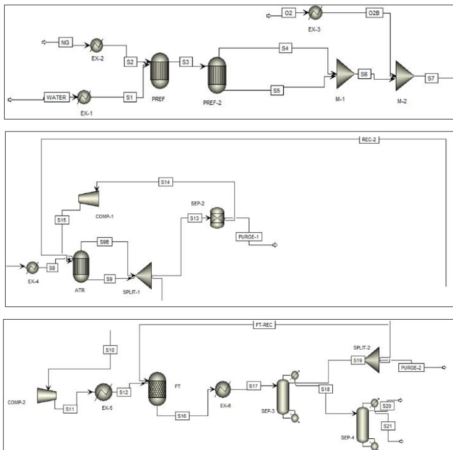
Fig 3: Flowsheet for the FT-GTL Synthesis Simulation
