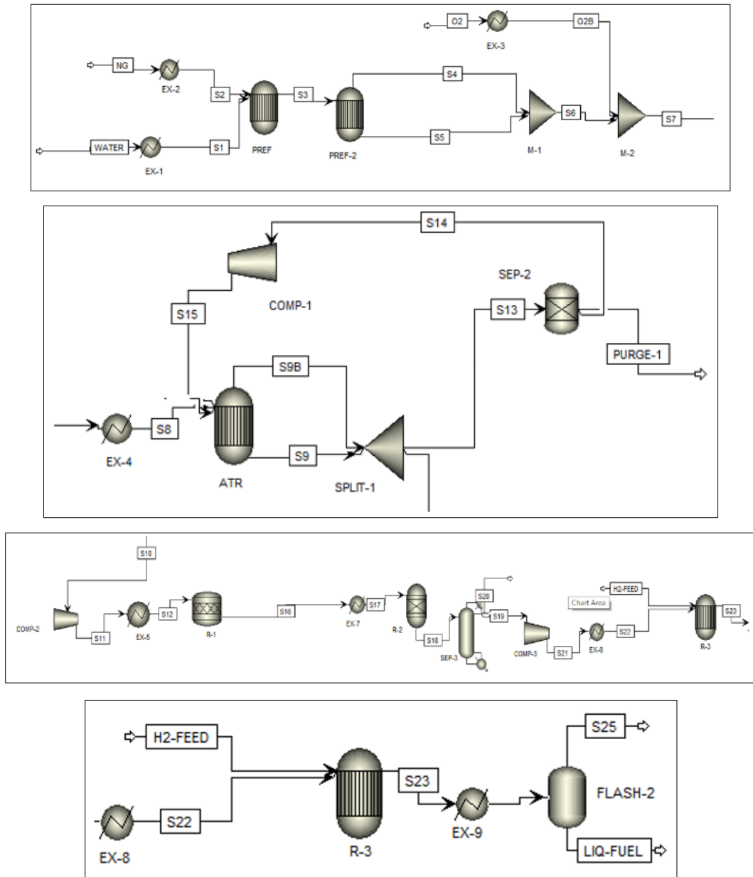
Fig 4: Flowsheet for the Bio-GTL Synthesis Simulation
