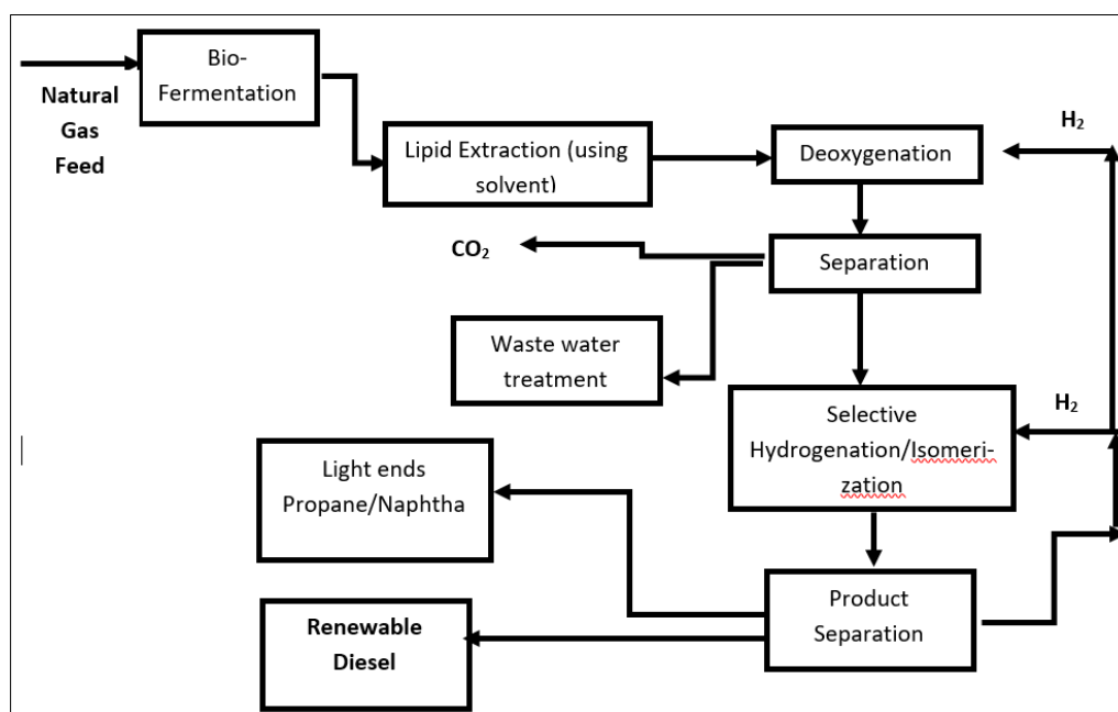
Fig 1: Bio-GTL Process routes
