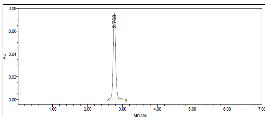
Fig 3: Optimized Chromatogram for Dolutegravir
