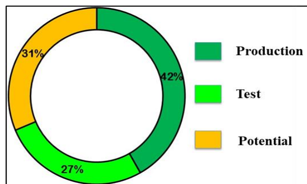
Fig 7: The Status Of Basement Reservoir
