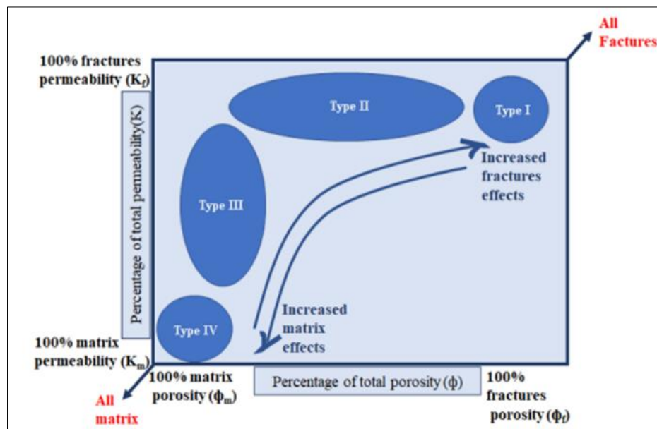
Fig 9: Classification of the naturally fractured reservoir based on percent of total permeability and porosity of the matrix and fractures
