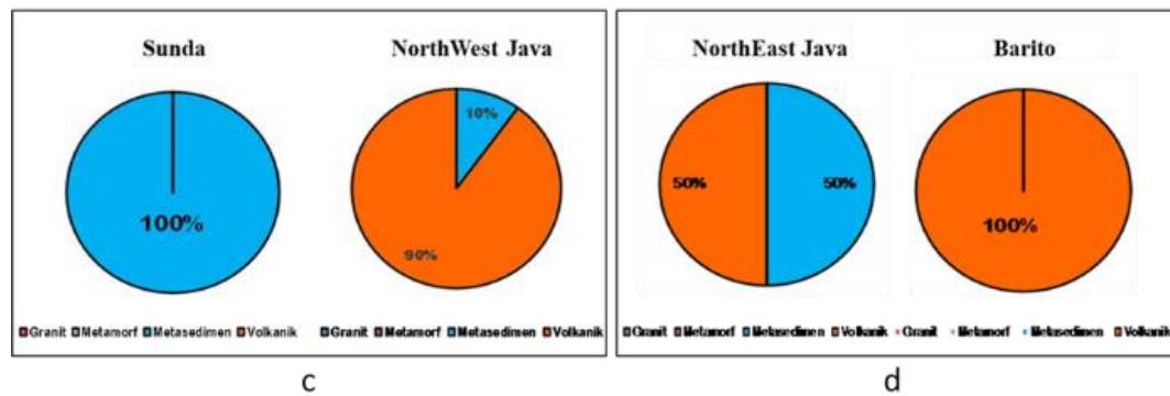
Fig 6: Lithology Variation of Basement Reservoir in each Basin
