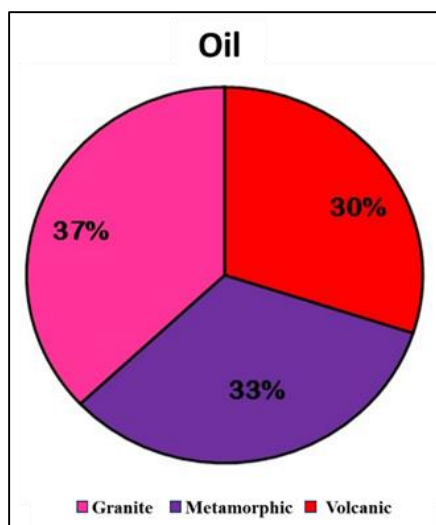
Fig 12: Oil Content in Basement Reservoir
