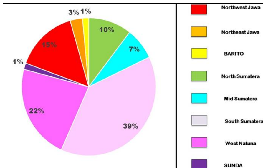
Fig 4: Basin With Basement Reservoirs
