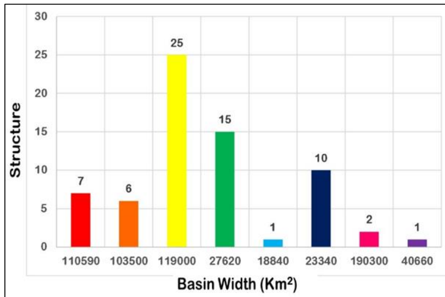
Fig 3: Basin Width Versus Structure
