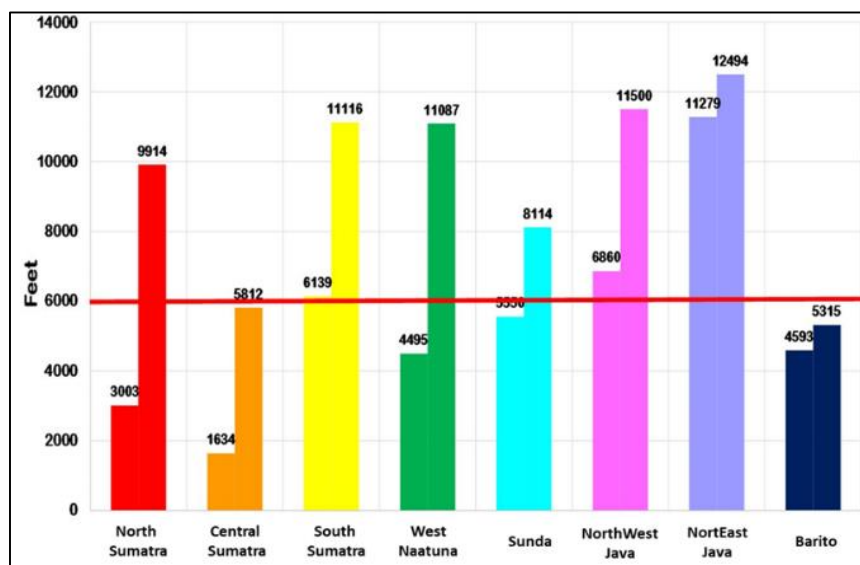
Fig 5: The Depth of Basement Reservoirs
