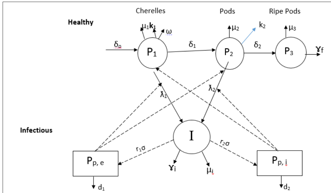
Fig 1: Schematic diagram of Cocoa black pod transmission
