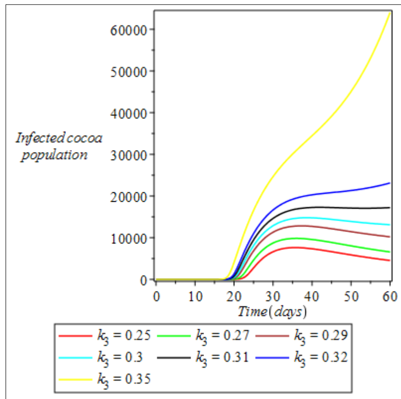
Fig 3: Graph of I(t) with control against t
