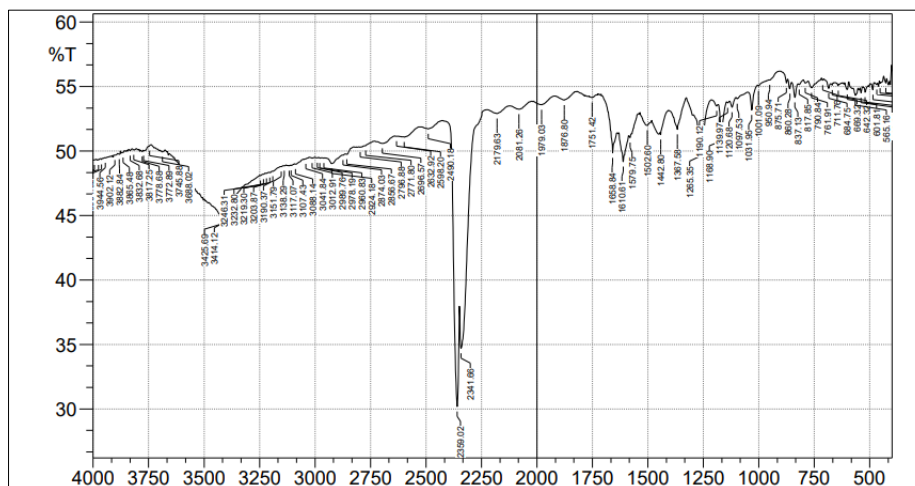
Fig 1: FTIR Spectra of Methylphenidate
