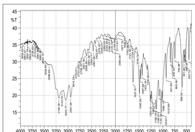
Fig 2: FTIR Spectra of Optimized formulation
