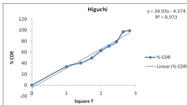
Fig 7: Higuchi model of Optimized formulation
