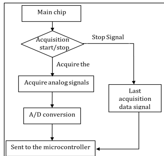
Fig 8: Sensing module subroutine flowchart
