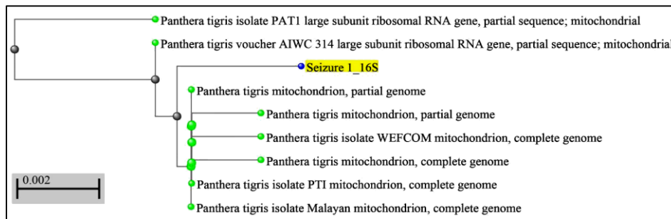
Fig 6: Seizure 1 BLAST tree view generated upon pairwise alignments using 16S rRNA on the NCBI database
