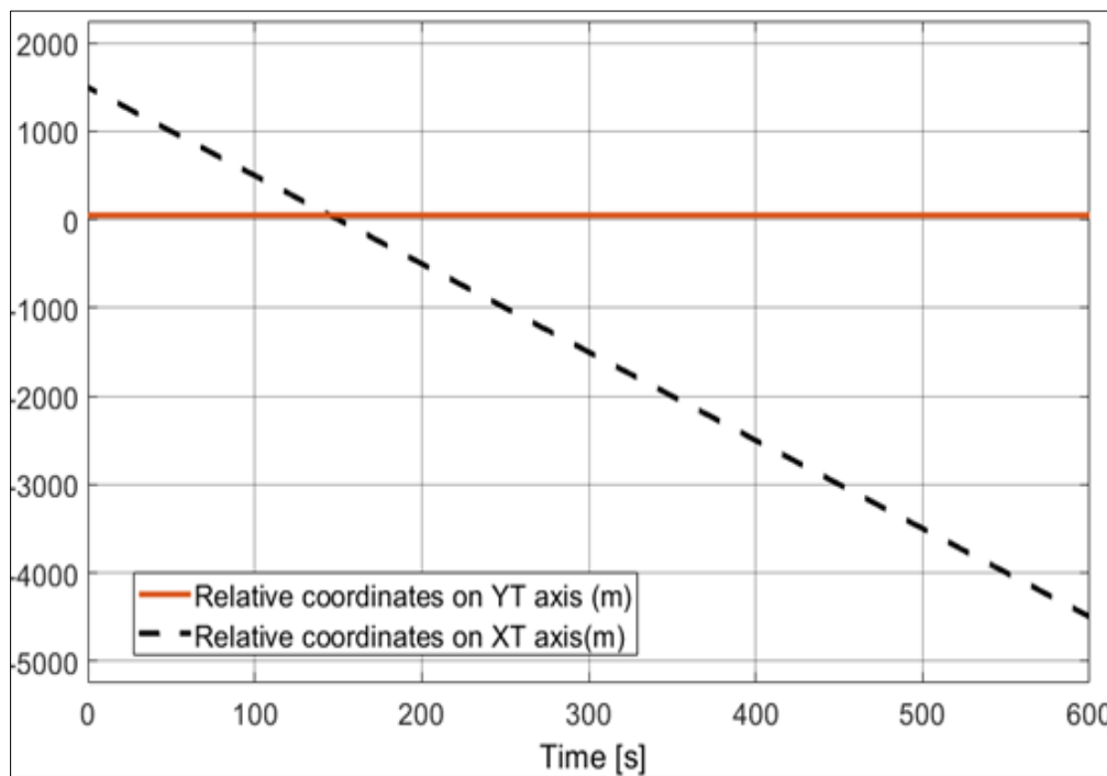
Fig 9: Relative coordinates of the reference point relative to the UAV in the UAV body coordinate system when the trajectory is a straight line.
