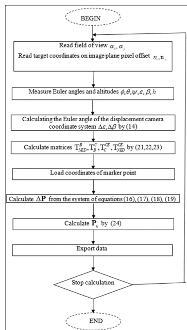
Fig 3: Flowchart of the algorithm to determine the coordinates of the UAV from the camera and the marker
