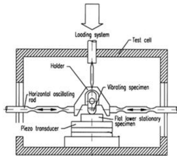
Fig 3: High Frequency Test Device
