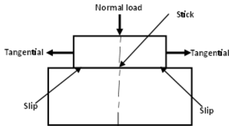
Fig 1: Stick and slip zones at fretting contact
