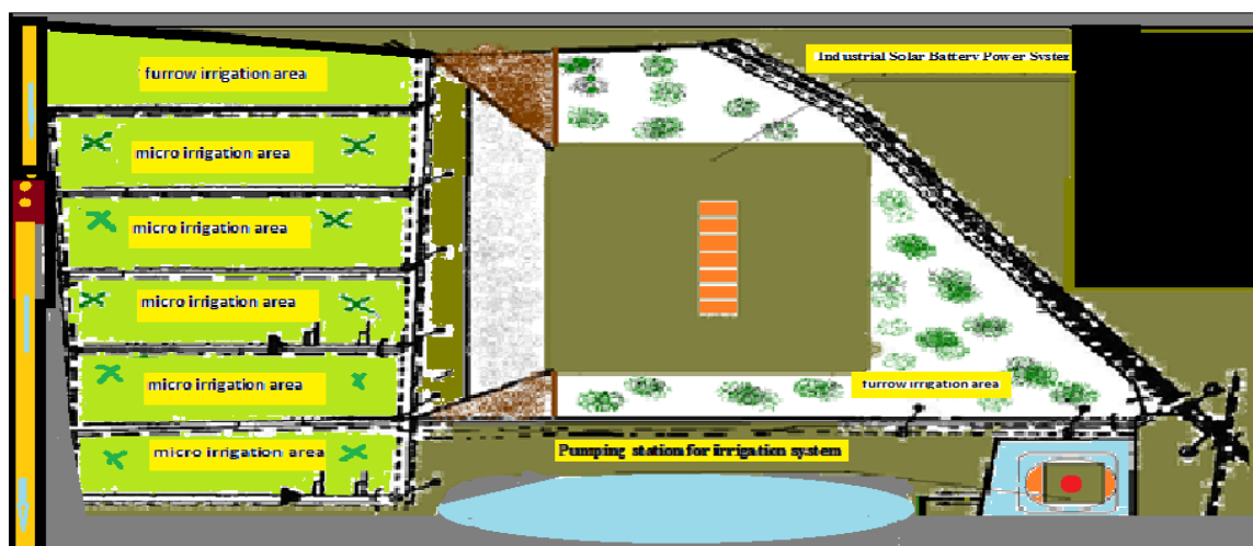
Fig 2: Scheme of the irrigation sprinkling station on the experimental part of the Terter RACS in the Garabagh land in the period 2006-2010 with the use of the Idad and MDR sprinklers:
