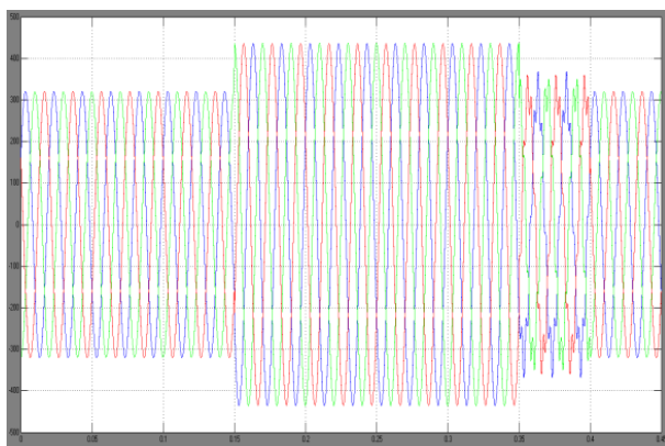
Fig 4.11: Source voltage during swell and harmonics
