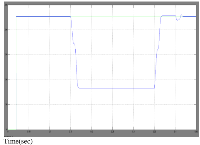
Fig 4.3: Source and load RMS voltages V_{srms} and V_{srms} during sag and harmonics
