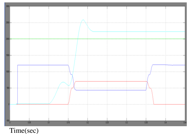
Fig 4.9: Active power of grid, load, and inverter during voltage sag and harmonics
