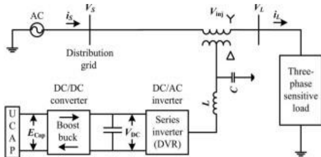
Fig 1.1: Single Line Diagram of DVR with UCAP energy storage system.
