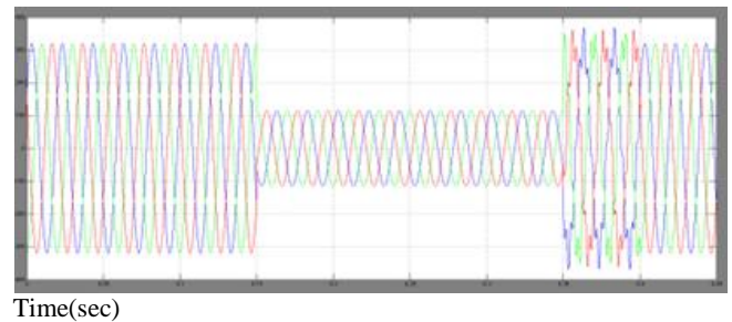
Fig 4.4: Source voltage during sag and harmonics
