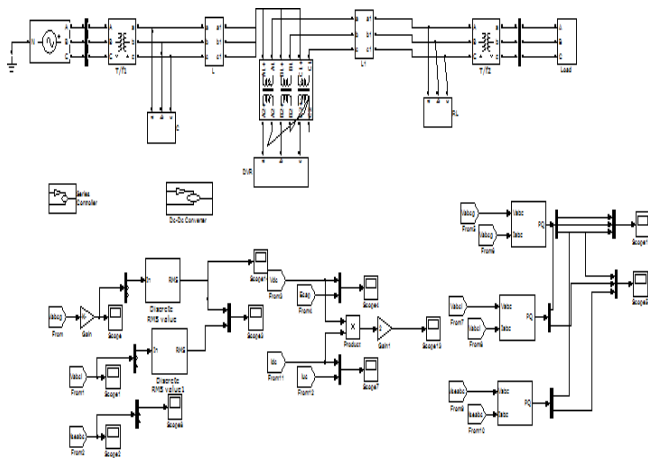
Fig 4.1: Simulink Model of Proposed system
