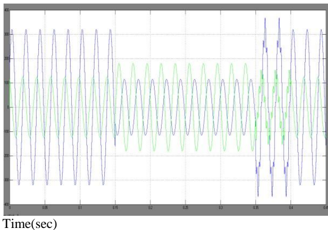
Fig 4.7: Vinj2a and Vsub2a waveforms during sag and harmonics.
