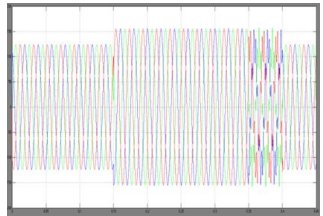
Fig 4.13: Injected voltage during swell and harmonics
